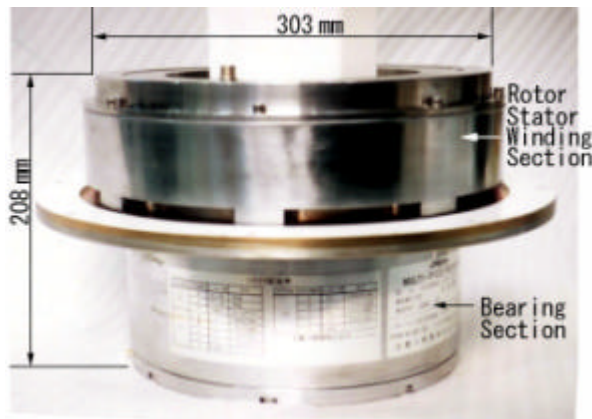
Figure 1. A newly developed resolver with an accuracy of 30 mas rms
