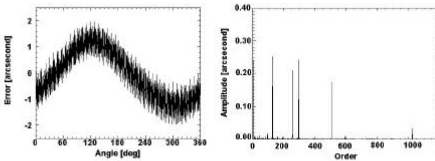
Figure 3. Measurement of raw readout of the azimuth encoder (left) and its Fourier components (right)
