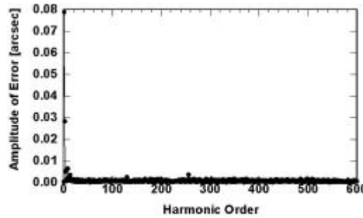
Figure 5. Fourier components of error due to shaft radial misalignment of 0.10 mm
