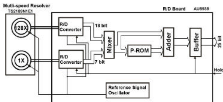
Figure 2. A block diagram of a resolver-to-digital converter system
