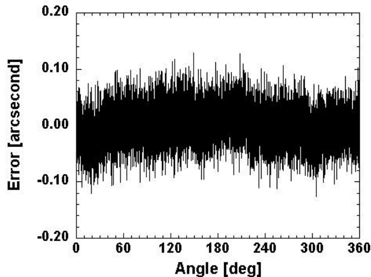
Figure 4. Angle errors of readouts after PROM compensation
