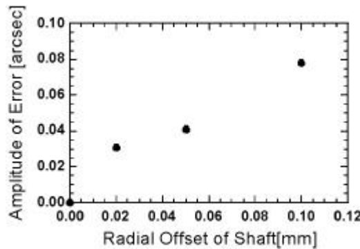
Figure 6. Increase of error due to shaft radial misalignment
