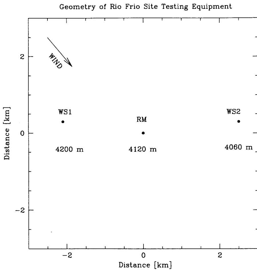
Figure 1: Geometrical layout of the Rio Frio site testing equipment: WS1 is weather station 1, WS2 is weather station 2, and RM is the radio seeing monitor and radiometer. Winds are generally from the northwest. Positions have been taken from Nakai's revised map.
