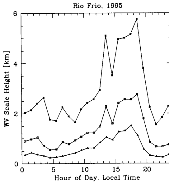
Figure 6: First, second, and third quartiles of the water vapor scale height as a function of hour.
